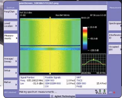
Interference analyzer
